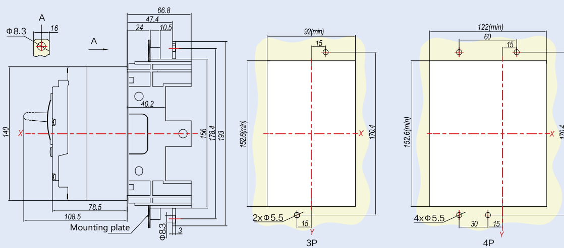
NM8N-125 Plug-in front connection
