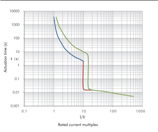
Tripping characteristic curve of motor protection
