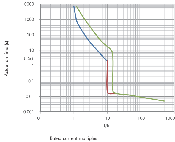
NXM-1250, 1600
