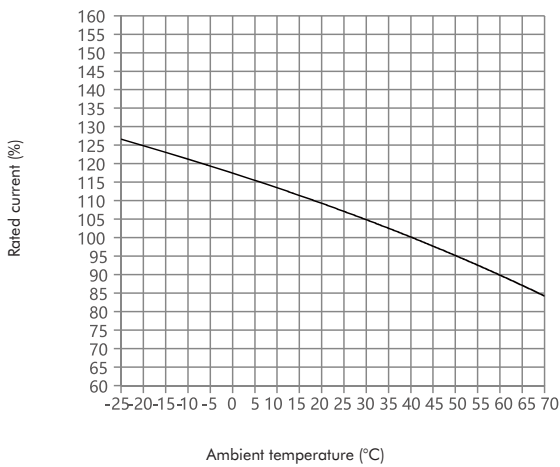
NXMLE-125 32A~63A
