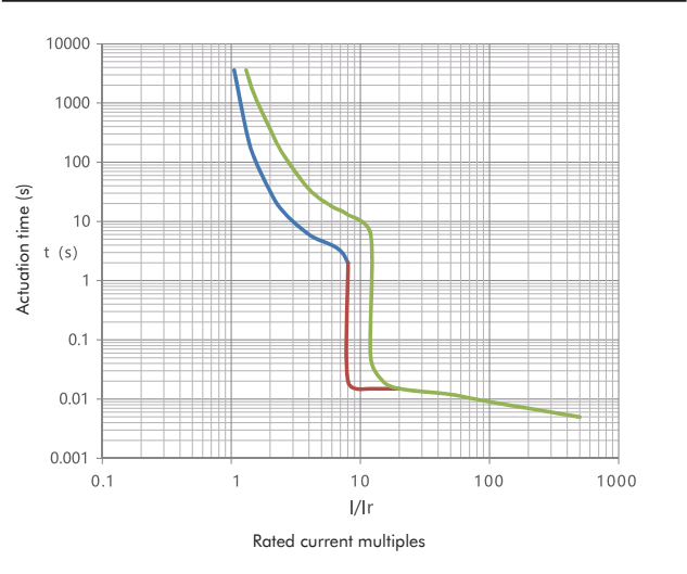
Tripping curve
