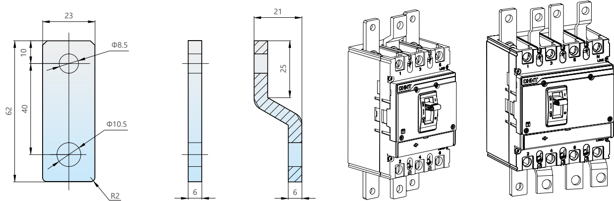
Coupling plates, dimension (mm)
