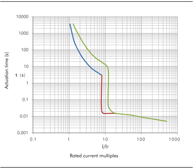
Tripping curve
