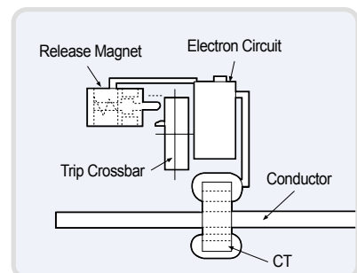
Fig. B-5. Electronic electric type trip unit
