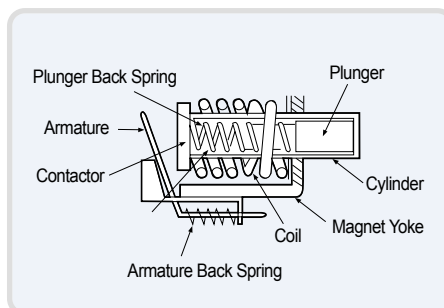
Fig. B-4. Hydraulic-magnetic type trip unit
