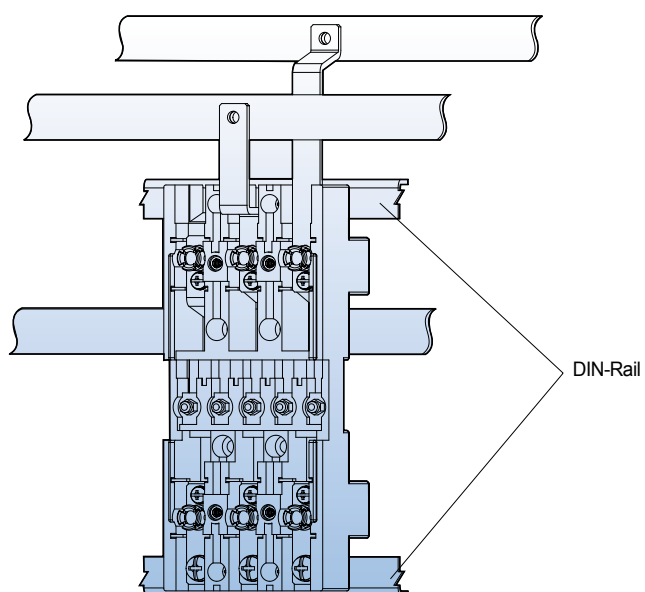
[Installing on the front of the mounting rail]
