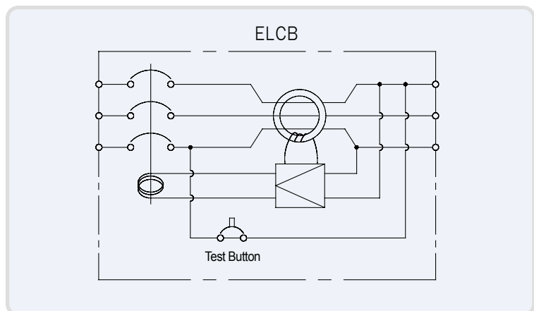
Fig. B-11. Test device circuit
