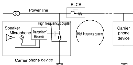
Fig. G-3. Example of carry phone device installation
