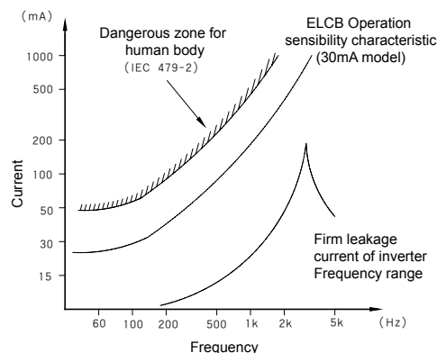
Fig. G-6. How to determine the characteristic of ELCB frequency
