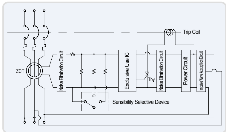
Fig. B-9. Electronic circuit unit
