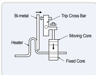
Fig. B-3. Thermal-magnetic type trip device
