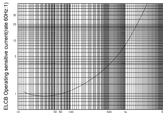
Fig. G-5. Characteristic of ELCB frequency
