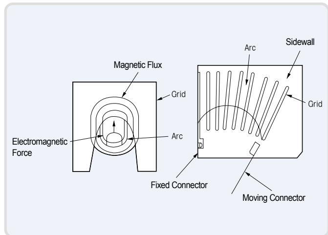
Fig. B-7. Effect of magnetic field
