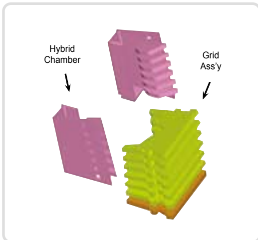
Fig. B-6. Arc-extinguishing unit
