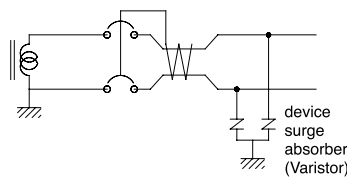
Fig. G-4. Example of surgy absorber installation
