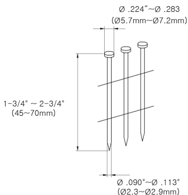
1 Roll (225~300pcs) Smooth, Ring, Screw Type
