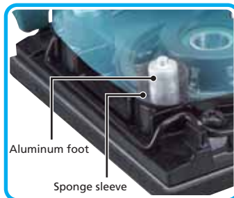
Rigid aluminum foot with dust-proof sponge for longer tool life
