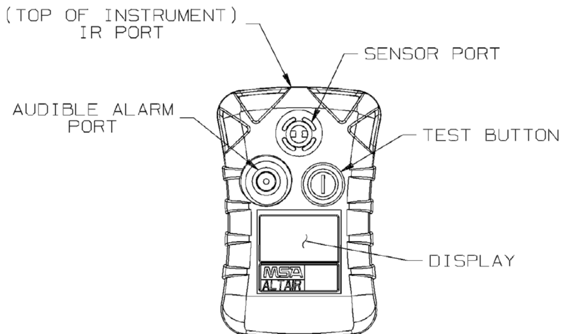
Figure 1 ALTAIR Overview
