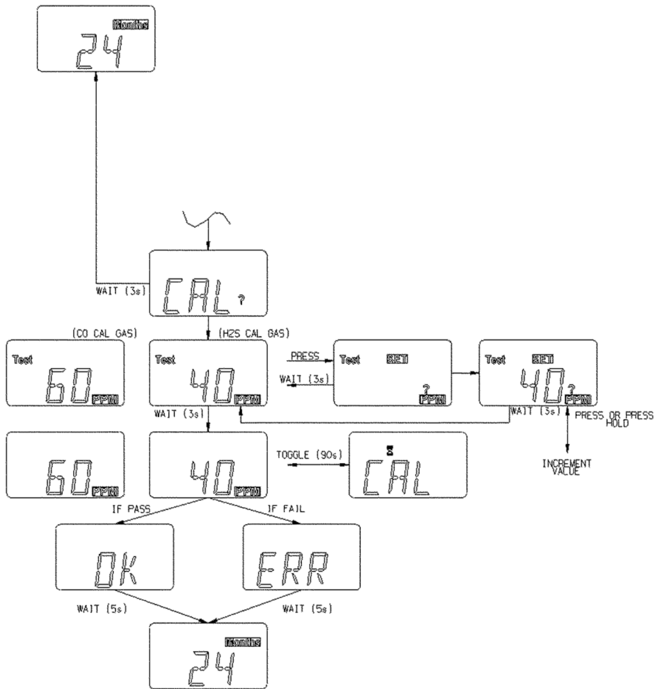
Figure 8 Calibration (Toxics) Flow Chart (part 2 of 2)
