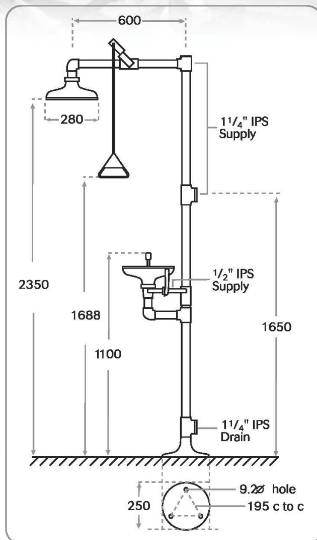
Stainless Steel Bowl Combination Emergency Shower & Eyewash with Foot Pedal
